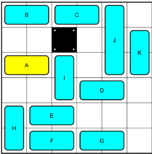
19 Moves_No193244.png
